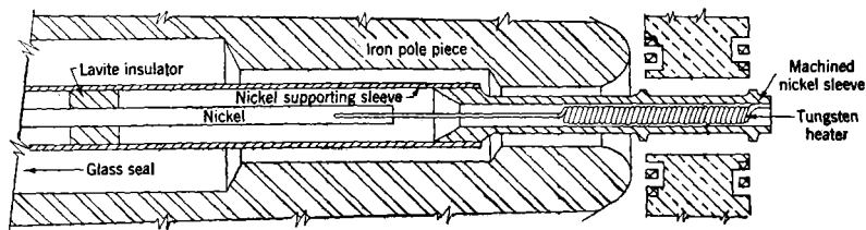
FIG. 12-29.—Oxide screen cathode of the 2J42. (2½×.)
